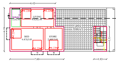
PRO.FIRST FLOOR PLAN
