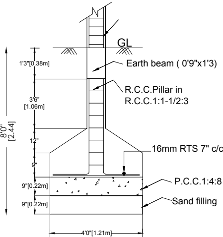
FOUNDATION DETAILS
