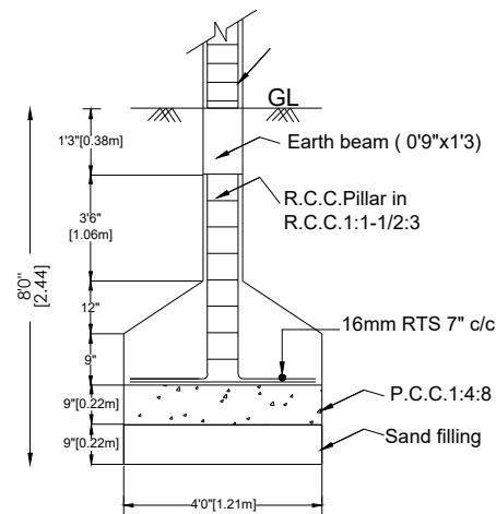
FOUNDATION DETAILS
