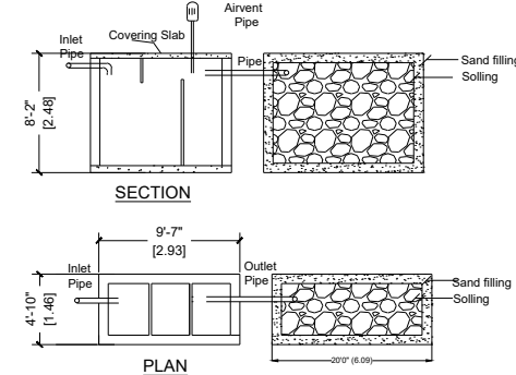
DETAILS OF SEPTIC TANK & DISPERSION TRENCH
