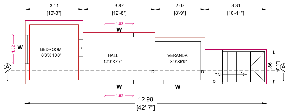
PRO.FIRST FLOOR PLAN
