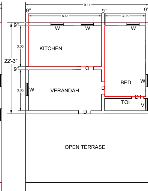
PROPOSED F.F. PLAN
