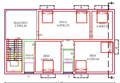
PRO.FIRST FLOOR PLAN
