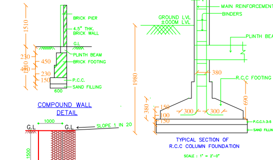
TYPICAL SECTION OF R.C.C. COLUMN FOUNDATION SCALE : 1" = 2'-0"
