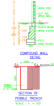
SECTION OF PEBBLE TRENCH SCALE: 1"=100
