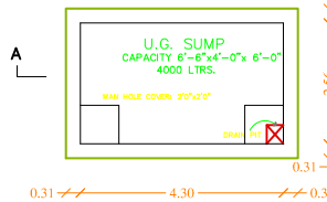
SUMP DETAIL SCALE 1"=4'-0"
