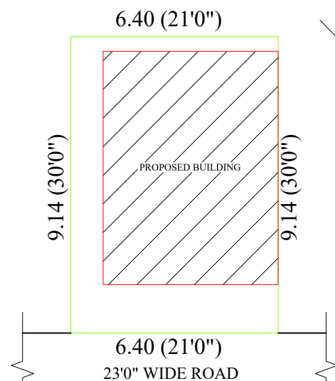
SITE PLAN
