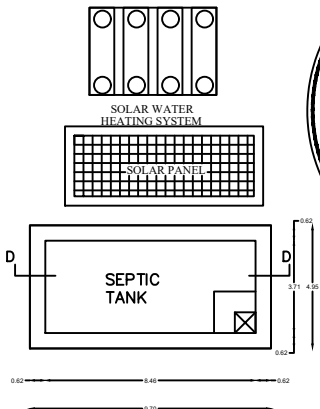
PLAN OF SEPTIC TANK SCALE 1"=2'-0"
