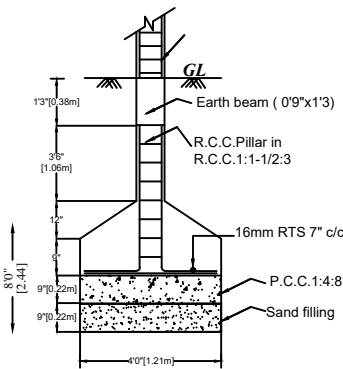
FOUNDATION DETAILS
