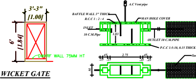
SEPTIC TANK AND TRENCH
