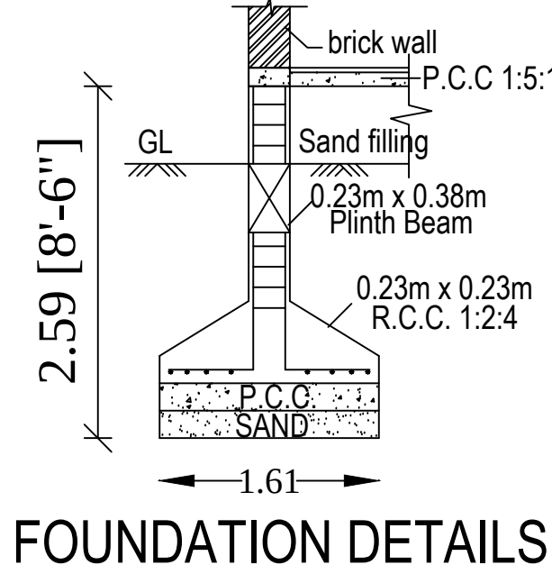
FOUNDATION DETAILS
