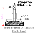
Isolated Footing - A (1.50X1.50) (Not To Scale)
