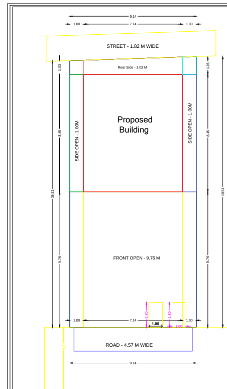
SITE BOUNDARY & PROPOSED SKETCH
