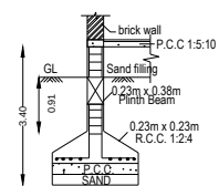
FOUNDATION DETAILS
