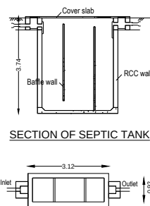
PLAN OF SEPTIC TANK
