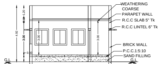
SECTION ON A-B
