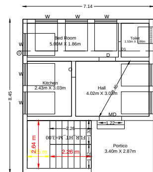
PROPOSED GROUND FLOOR
