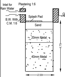
RAIN WATER PERCOLATION PIT
