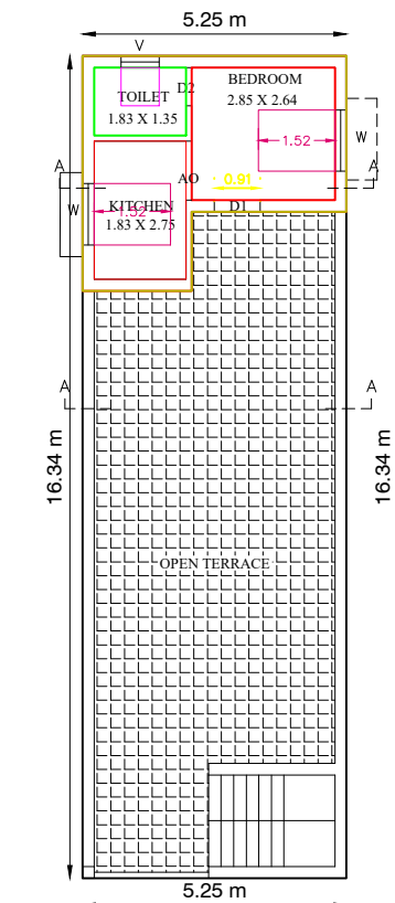
PRO. FIRST FLOOR PLAN
