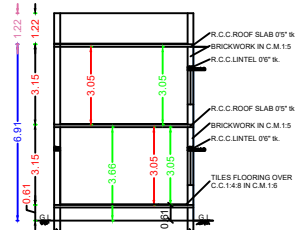
SECTION ON B-B
