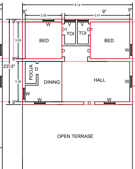
PROPOSED SECOND FLOOR
