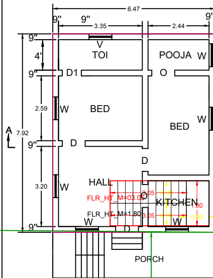
EXISTING G.F. PLAN
