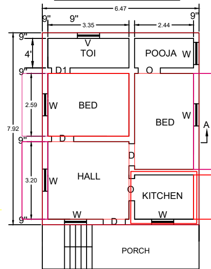
PROPOSED F.F. PLAN
