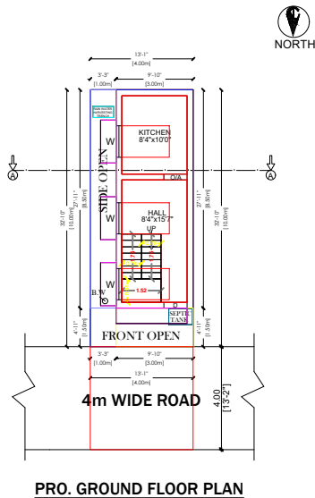
PRO. GROUND FLOOR PLAN
