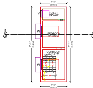
PRO. FIRST FLOOR PLAN
