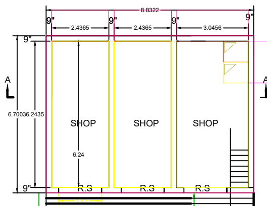
G.F. PLAN
