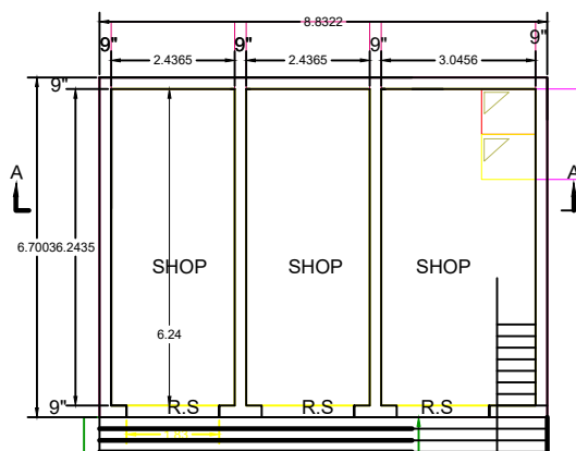
G.F. PLAN
