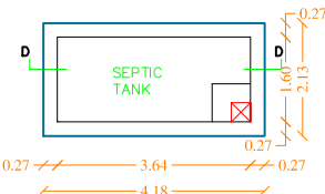
PLAN OF SEPTIC TANK SCALE 1\"/>
