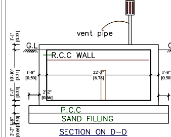
SECTION ON D-D
