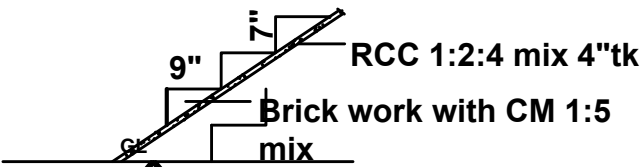
STAIRCASE DETAILS ( Not to Scale )
