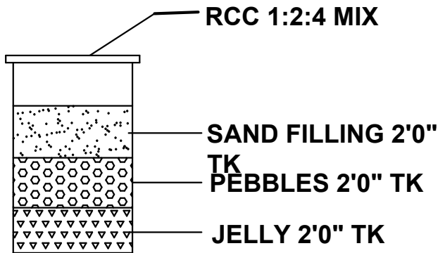
RAIN WATER HARVESTING TANK (Not to scale)
