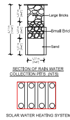
SECTION OF RAIN WATER COLLECTION PITS (NTS)
