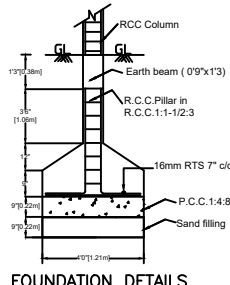
FOUNDATION DETAILS
