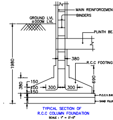
TYPICAL SECTION OF R.C.C. COLUMN FOUNDATION
