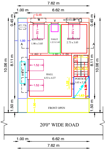
PRO.GROUND FLOOR PLAN
