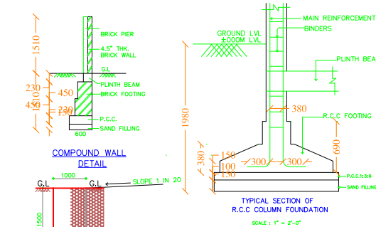
TYPICAL SECTION OF R.C.C. COLUMN FOUNDATION
