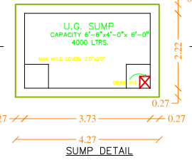
SUMP DETAIL
