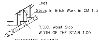
STAIRCASE DETAILS
