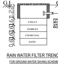
RAIN WATER FILTER TRENCH
