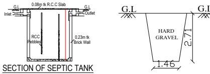
SECTION OF SEPTIC TANK
