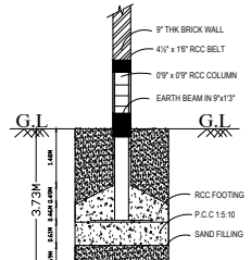
FOUNDATION DETAIL
