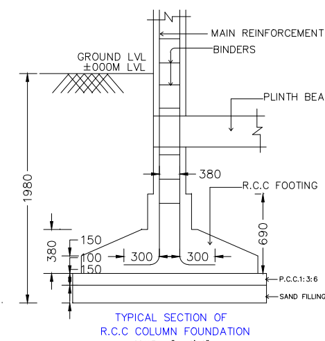
TYPICAL SECTION OF R.C.C. COLUMN FOUNDATION
