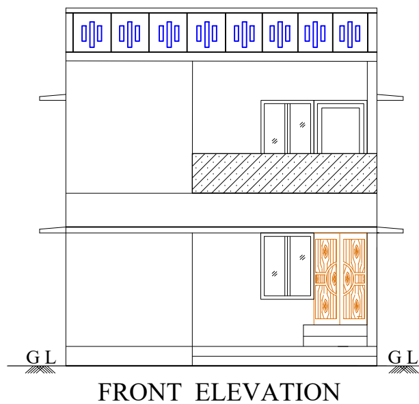
FRONT ELEVATION
