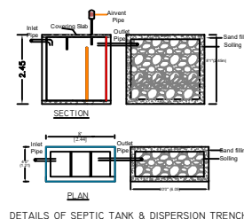
DETAILS OF SEPTIC TANK & DISPERSION TRENCH
