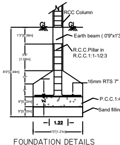
FOUNDATION DETAILS
