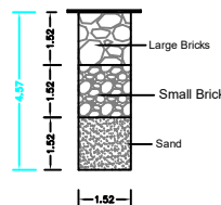
SECTION OF RAIN WATER COLLECTION PITS (NTS) RWH_CAPACITY_1 = 2000LTRS
