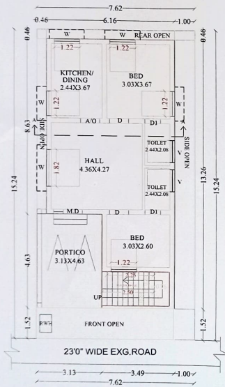
PRO-GROUND FLOOR PLAN
