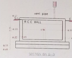
SECTION 09 D-D
