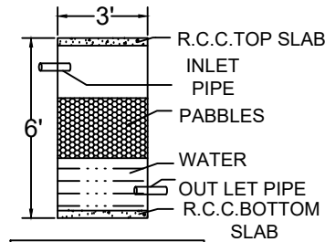
RAIN WATER TANK
