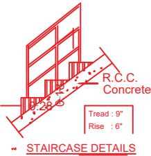
STAIRCASE DETAILS
