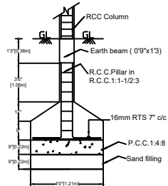
FOUNDATION DETAILS
