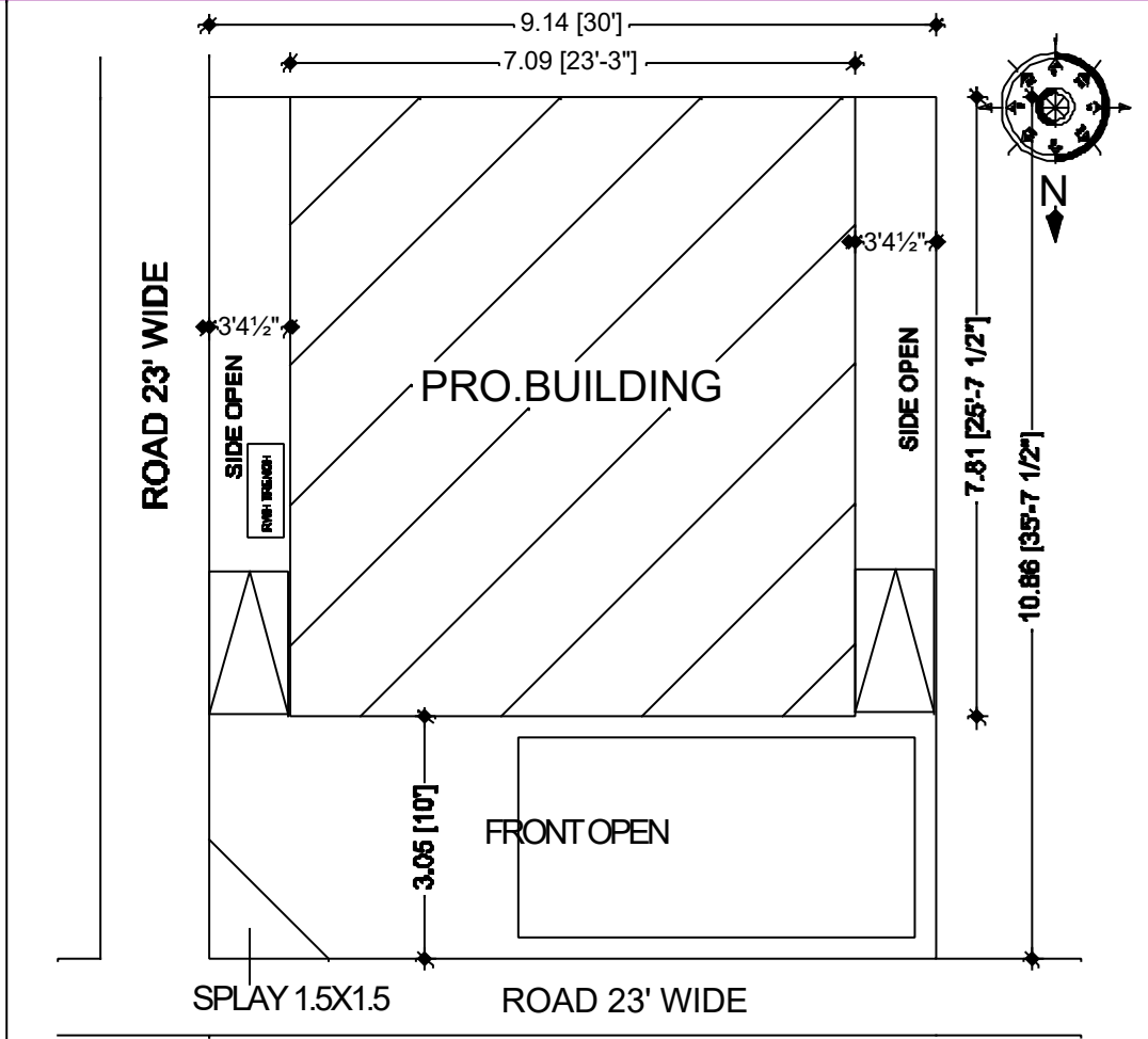
SITE-PLAN SITE-PLAN SHOWING R.S.No:76/1B4D1A1 & 76/1B4E, PLOT No:30, POTHUMBU VILLAGE I BIT, POTHUMBU VILLAGE PANCHAYAT, MDU.
