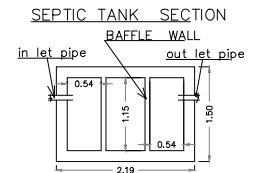
SEPTIC TANK PLAN
