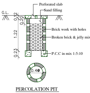
PERCOLATION PIT
