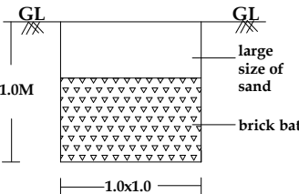
RAINWATER HARVESTING
