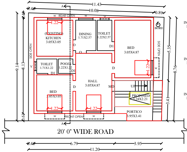
EXG & PRO.GROUND FLOOR PLAN
