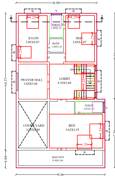
PRO.FIRST FLOOR PLAN
