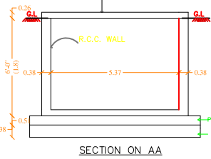
SECTION ON AA
