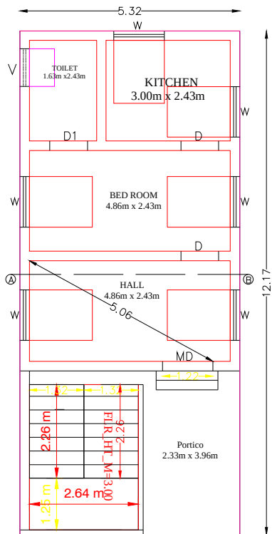
PROPOSED GROUND FLOOR
