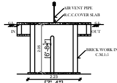
SEPTIC TANK DEATILS-SECTION
