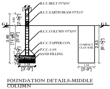
FOUNDATION DETAILS-MIDDLE COLUMN
