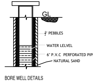
BORE WELL DETAILS
