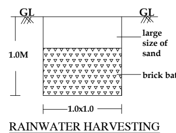
RAINWATER HARVESTING
