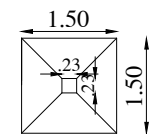
COLUMN FOUNDATION
