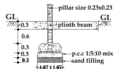
FOUNDATION DETAILS
