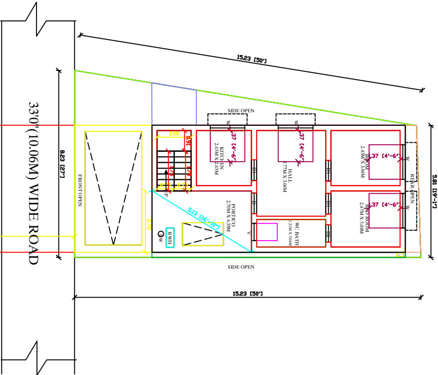
RAIN WATER FILTER TRENCH FOR GROUND WATER SAVING SCHEME
