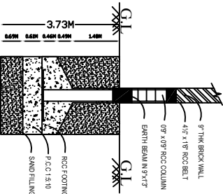
FOUNDATION DETAIL
