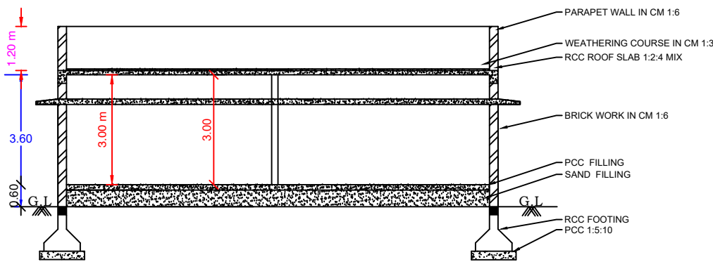
SECTION AB
