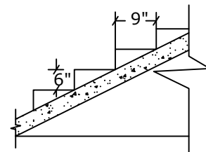
Staircase Detail Not To Scale
