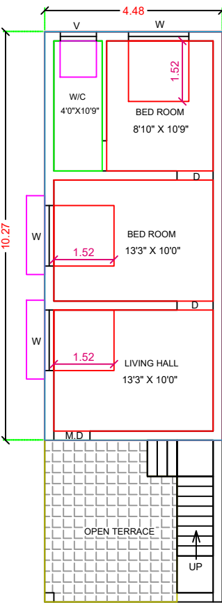
FIRST FLOOR PLAN (PROPOSED)
