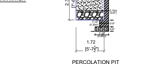
PERCOLATION PIT
