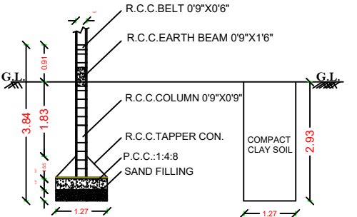
FOUNDATION DETAILS-MIDDLE COLUMN
