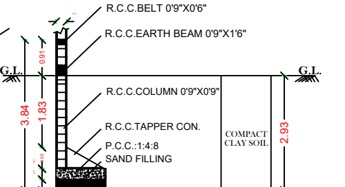
FOUNDATION DETAILS-END COLUMN
