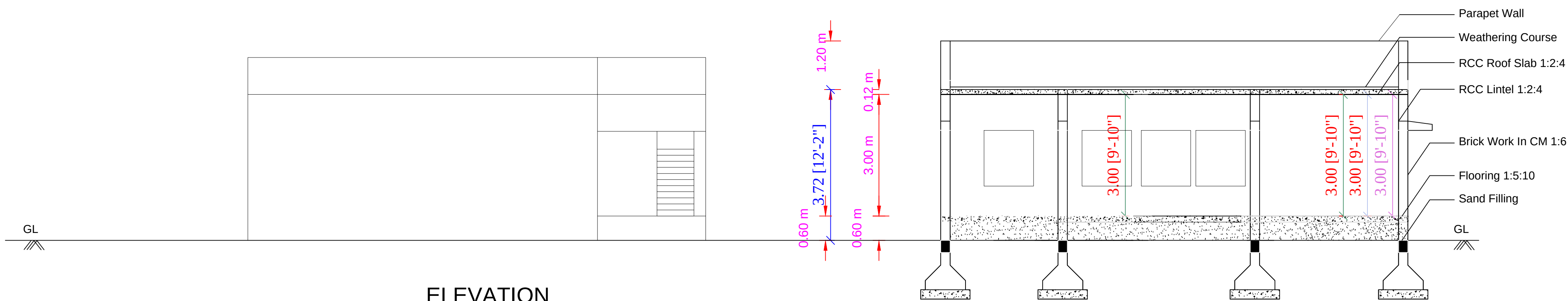
SECTION-AB
