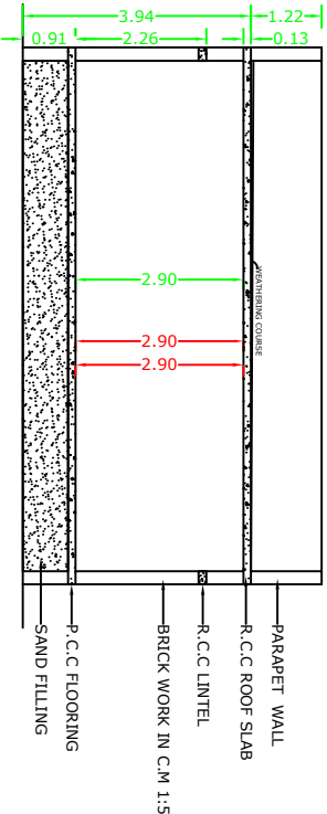
SECTION ON A - A
