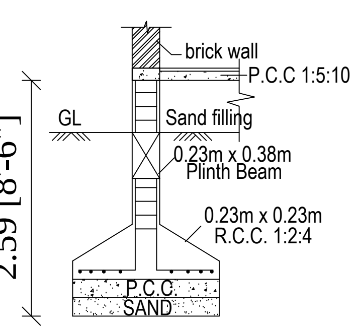
FOUNDATION DETAILS
