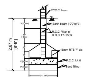
FOUNDATION DETAILS
